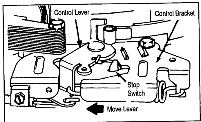
Control Lever, RUN Position
