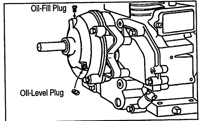
(Gear Reduction) Aluminum Engines Models 140000, 170000, & 190000
