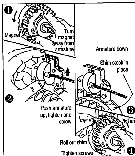
FLYWHEEL ARMATURE AIR GAP
