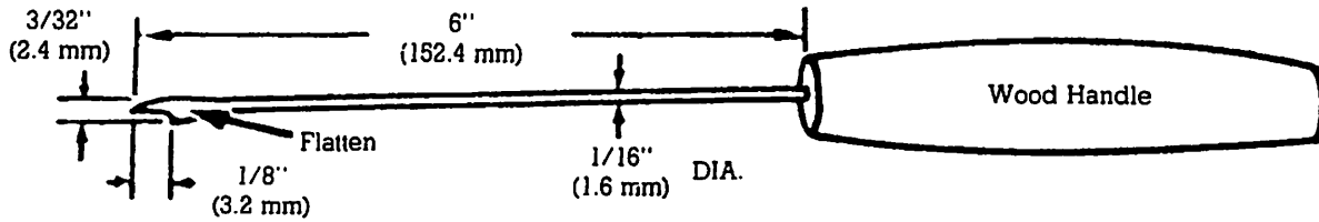
Rope Inserter
