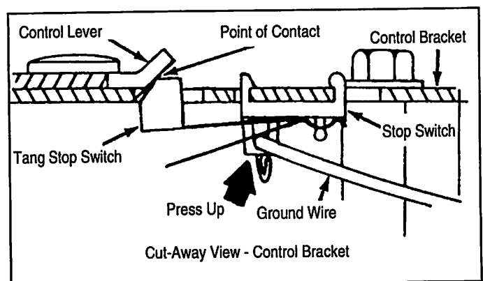
Control Lever - STOP Position
