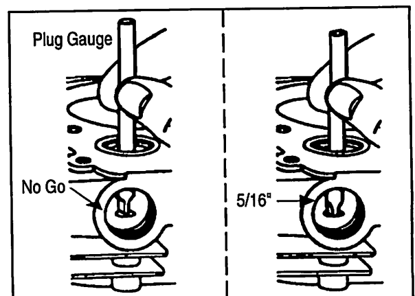
Plug Gauge 19122
