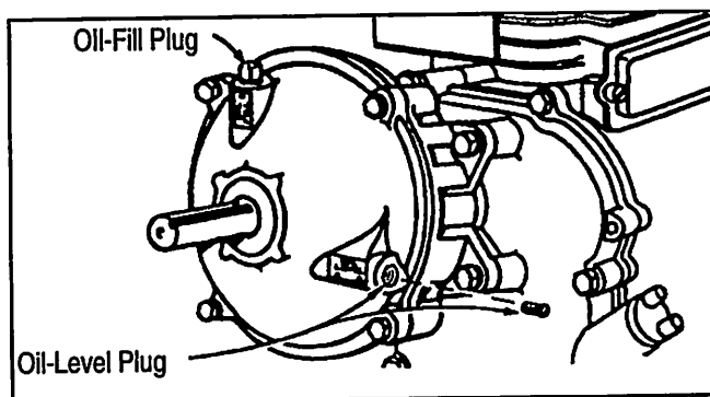
6 To 1 Gear Reduction Models 6,8, 60000, 80000, 100000, & 130000
