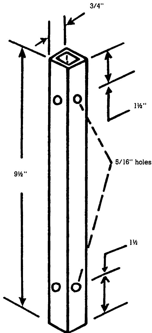
Rewind Starter Tool
