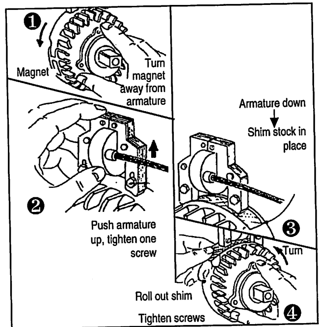
FLYWHEEL ARMATURE AIR GAP
